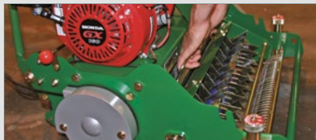
Lower cassette onto back tie bar and slide cassette across
