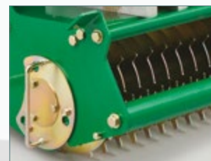
Simple changeover reel lock
