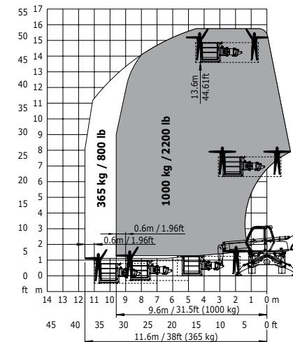
Rotation on lowered stabilisers with 365 kg platform
