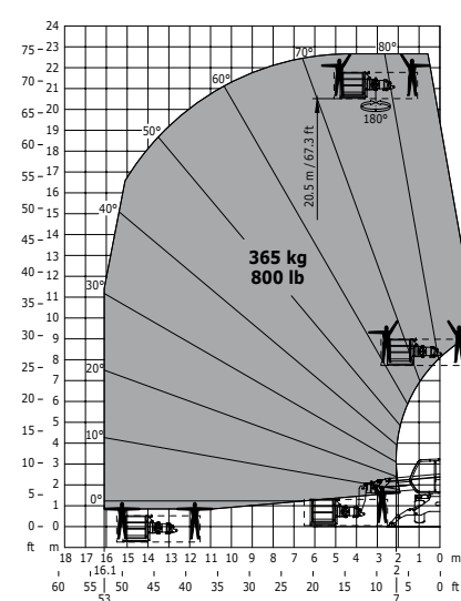
Rotation on lowered stabilisers with 365 kg platform
