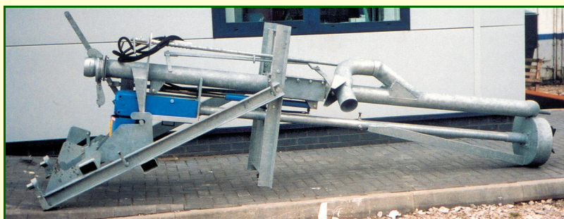
Powerflo variable depth pump, 8-10ft.
